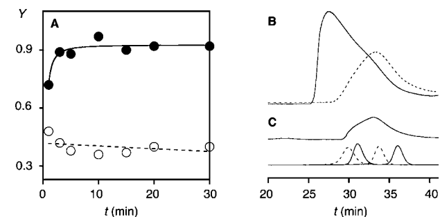
Figure 3. Polymers of 1 made with ( \bullet , solid) and without ( \circ , dashed) initiator 5 . (A) Y during polymerization of 1 (100 mM) with ( \bullet ) and without 5 ( \circ , 5 mM, pH 7). (B) GPC of 1 (100 mM) polymerized with (solid) and without 5 (dashed, 5 mM, pH 7), compared to (C) polyarginine (top) and standards (bottom, M_w 43, 25, 13.7, and 6.5 kDa); Superdex 75, 30% acetonitrile in acetate buffer, pH 6.5.
